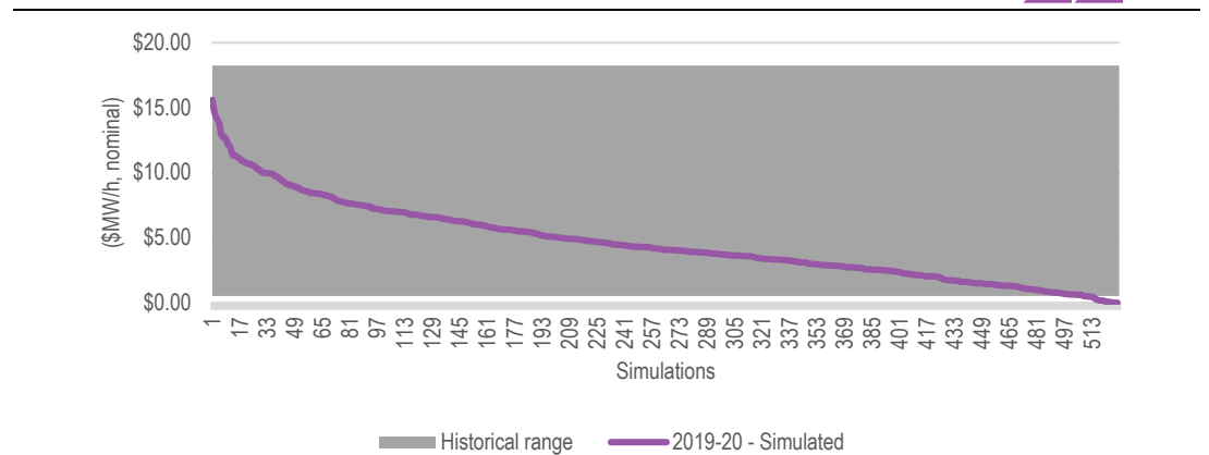
FIGURE 4.14 ANNUAL AVERAGE CONTRIBUTION TO THE QUEENSLAND TWP BY PRICES ABOVE $300/MWH FOR QUEENSLAND IN 2019-20 FOR 528 SIMULATIONS COMPARED WITH ACTUAL OUTCOMES IN PAST YEARS
