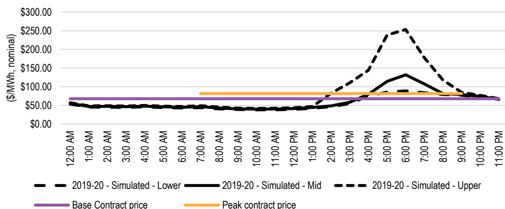
FIGURE 4.17 COMPARISON OF ANNUAL AVERAGE TIME OF DAY SIMULATED HOURLY PRICE CURVES FOR QUEENSLAND AND CONTRACT PRICES
